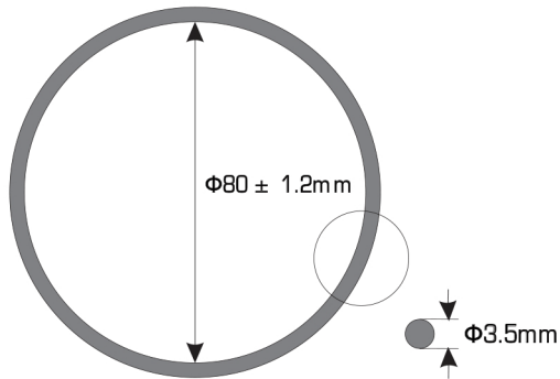
Gasket with Round Cross-Section
