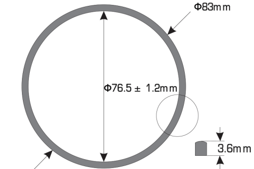
Gasket with "D"-Shaped Section
